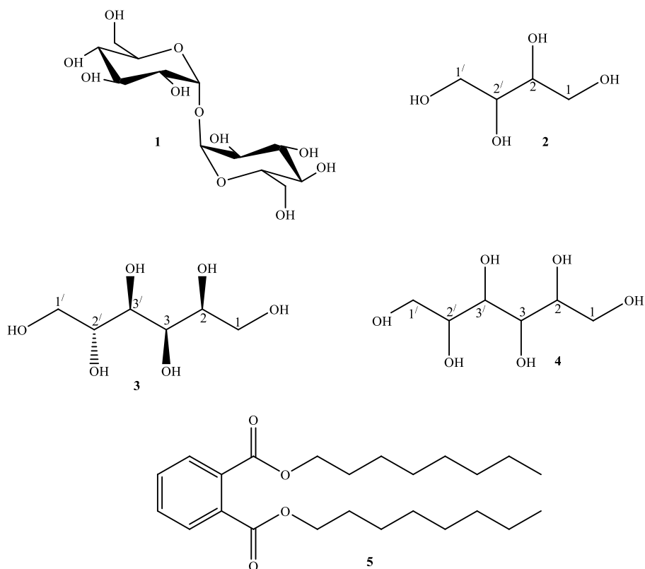
Figure 1. Structures of the compounds 1-5
