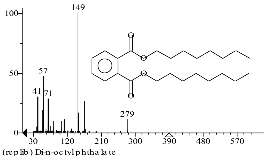
Figure 5. GCMS chromatogram of 5
