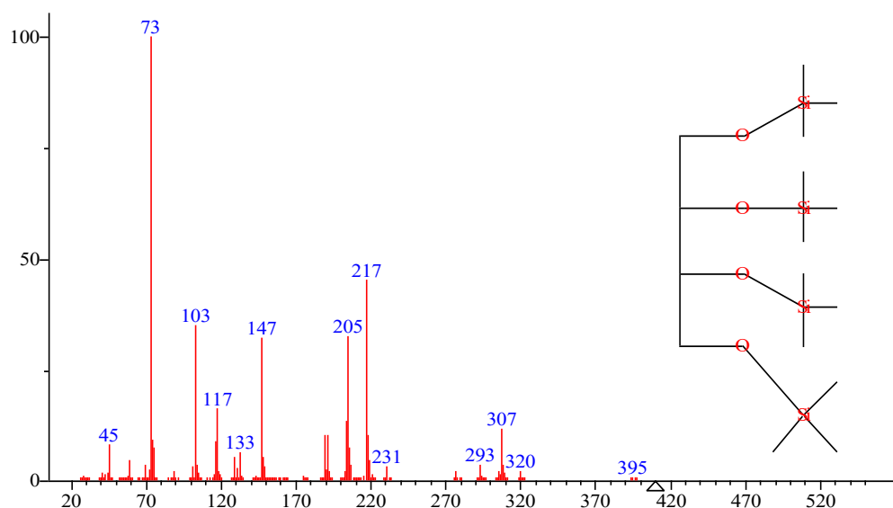
Figure 4. GCMS chromatogram of compound 2
